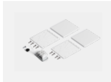
00-20102, B 2xend cap - plastic, 3- conductor terminal box, grommet
